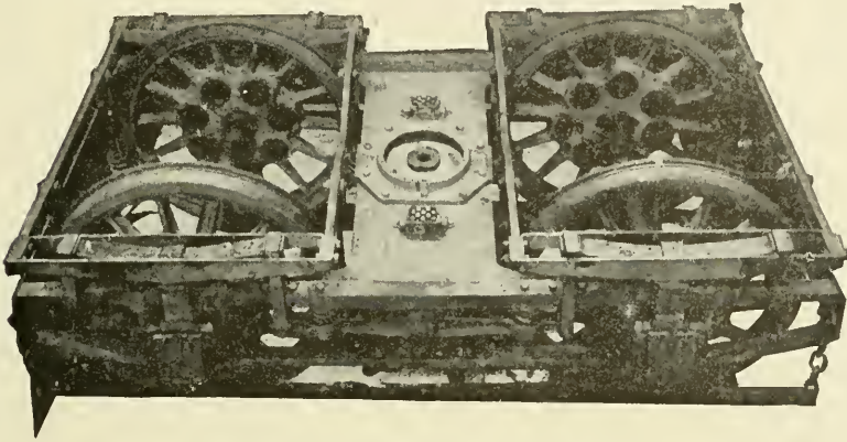
Fig. 255. View of Truck without Motors
